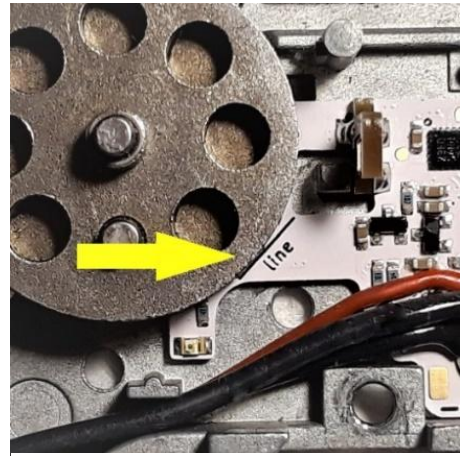
Sensor line and sector gear alignment
